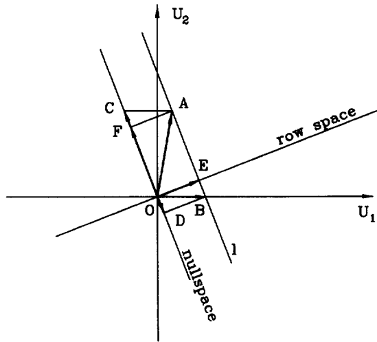
Fig. 1. Resolution of the displacements' modes.
