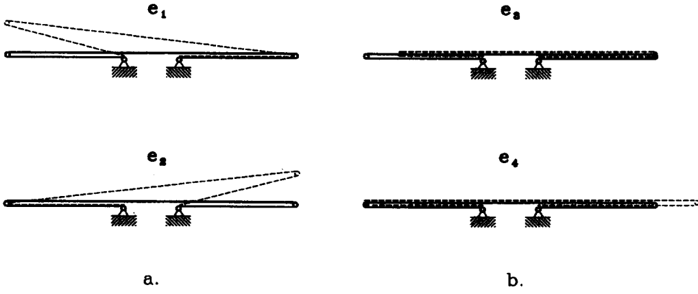
Fig. 4. "Kinematic" and "elastic" modes of displacements.
