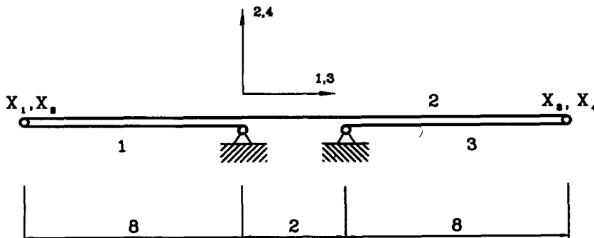
Fig. 3. Three-bars assembly.
